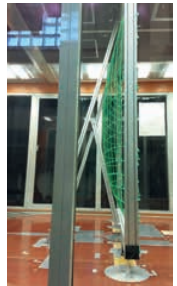
Test set-up to measure the wind load
